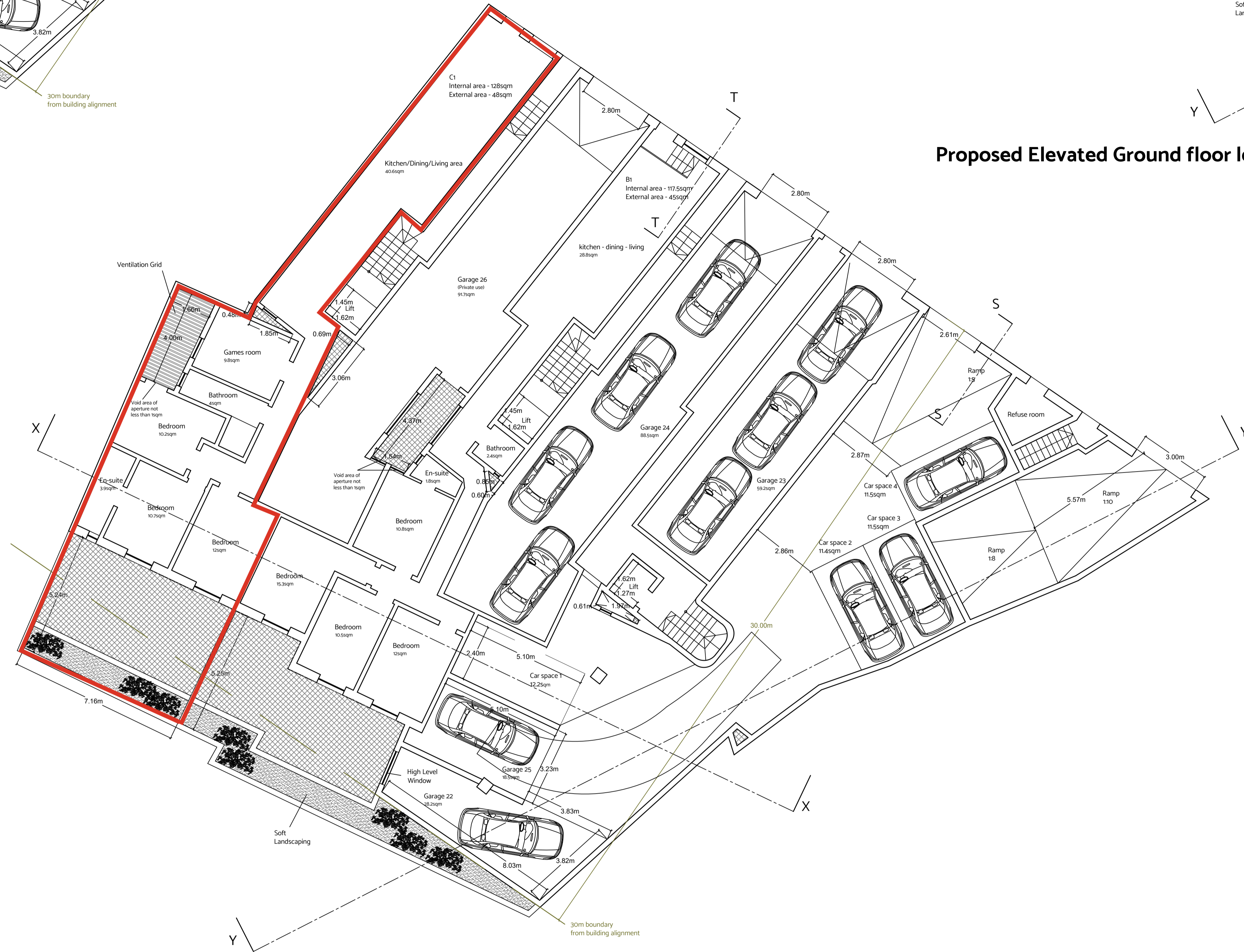
Proposed Elevated Ground floor level plan Scale 1:100 clean copy
