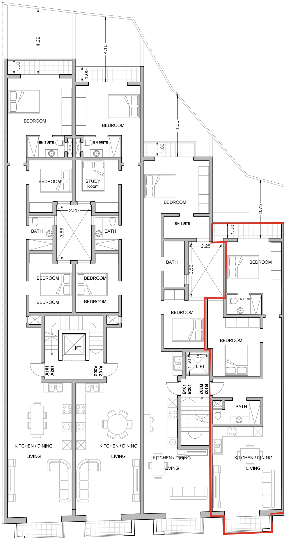
FIRST & SECOND FLOORS PROPOSED Scale 1:100
