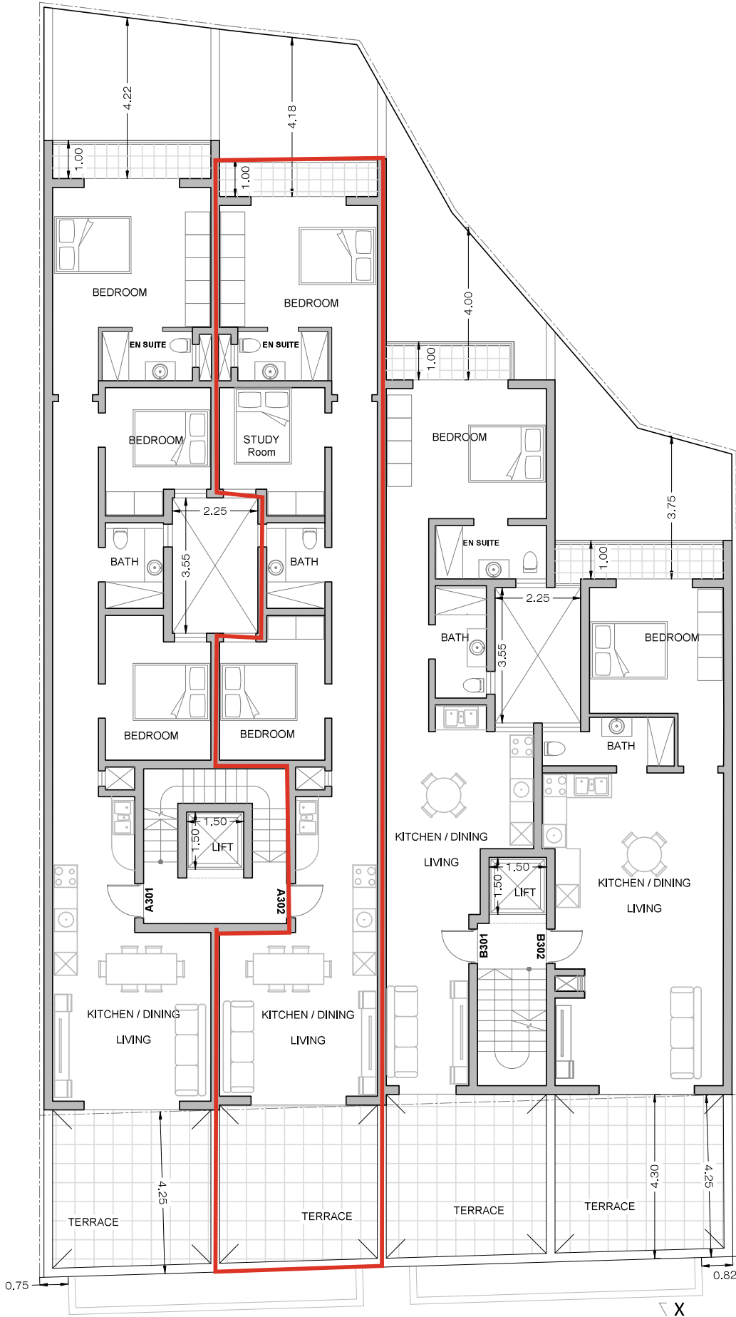
LOWER RECEDED FLOOR PROPOSED Scale 1:100
