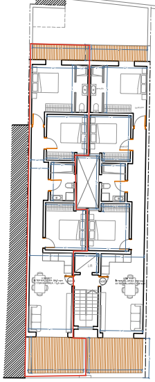
Proposed Floor Level 3 1:50 20/01/2020
