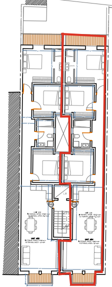
Proposed Floor Level 2 1:50 2024
