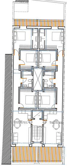
Proposed Floor Level 3 1:50
