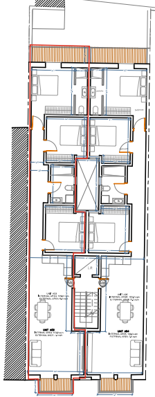
Proposed Floor Level 2 1:50
