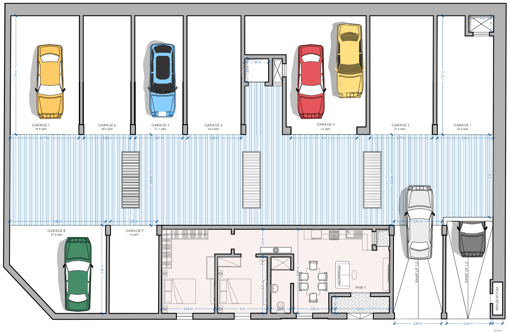
UPPER BASEMENT FLOOR PROPOSED SCALE 1:100
