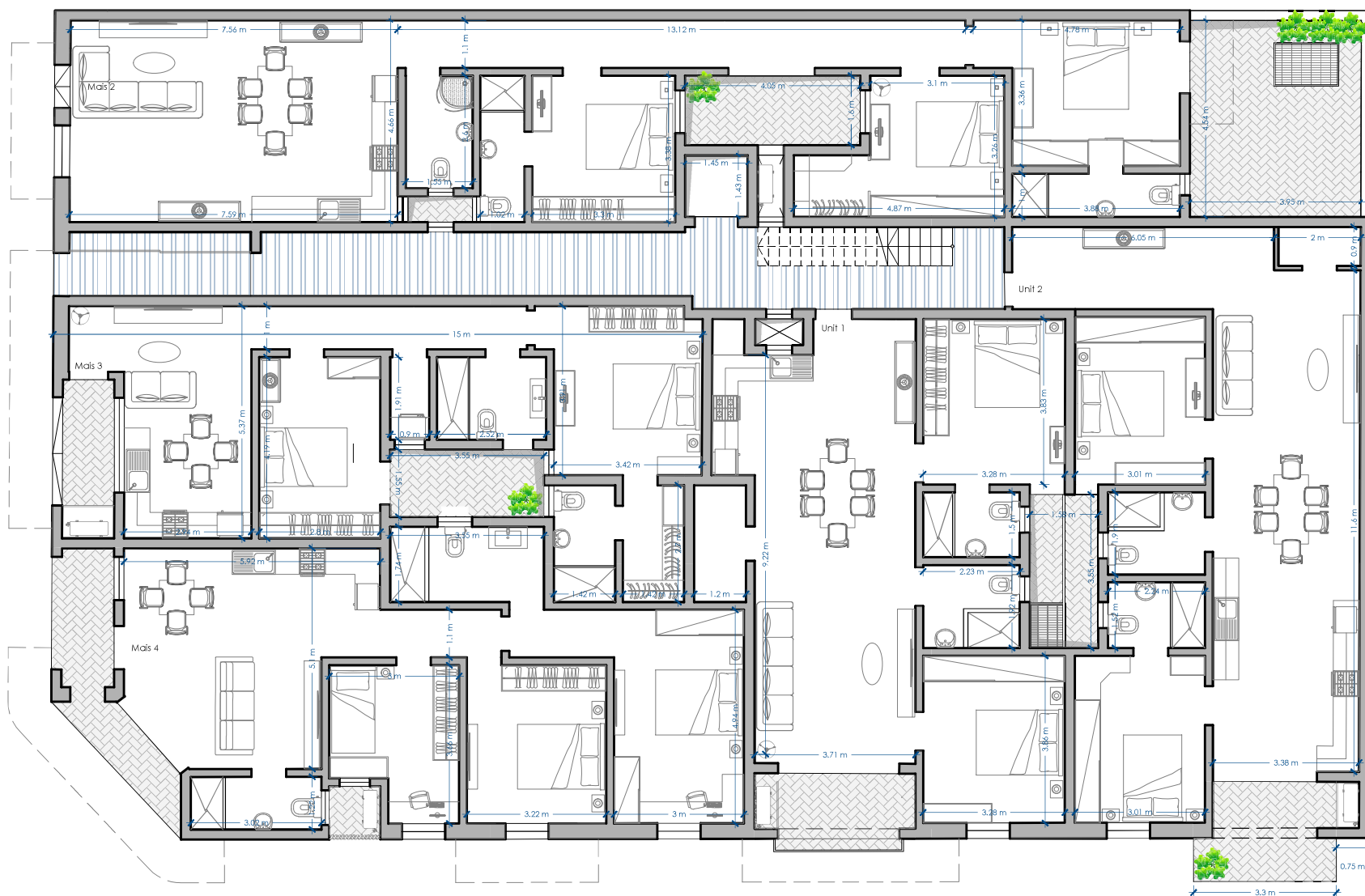
GROUND FLOOR PROPOSED SCALE 1:100
