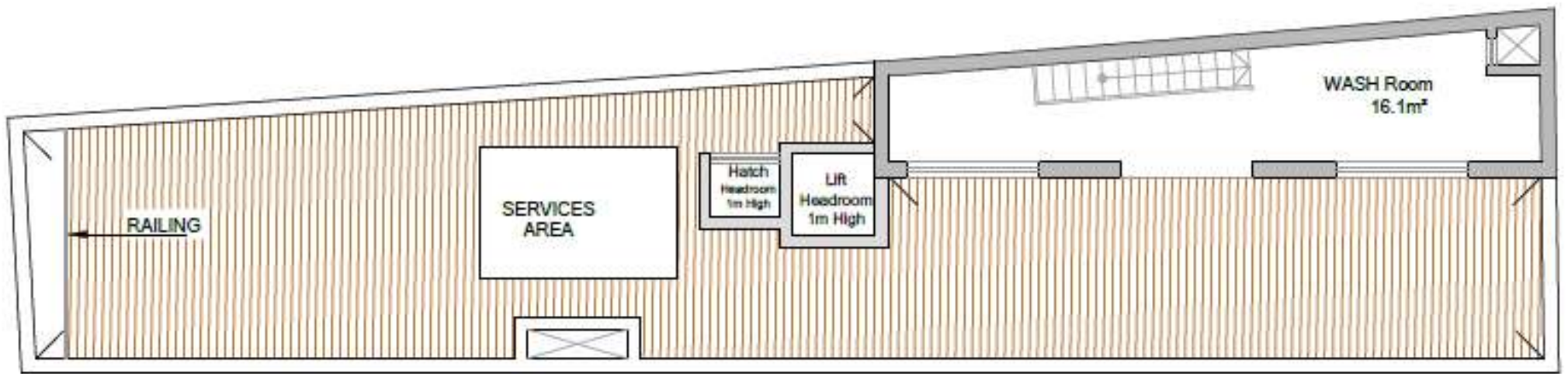
ROOF PLAN PROPOSED Scale 1:100
