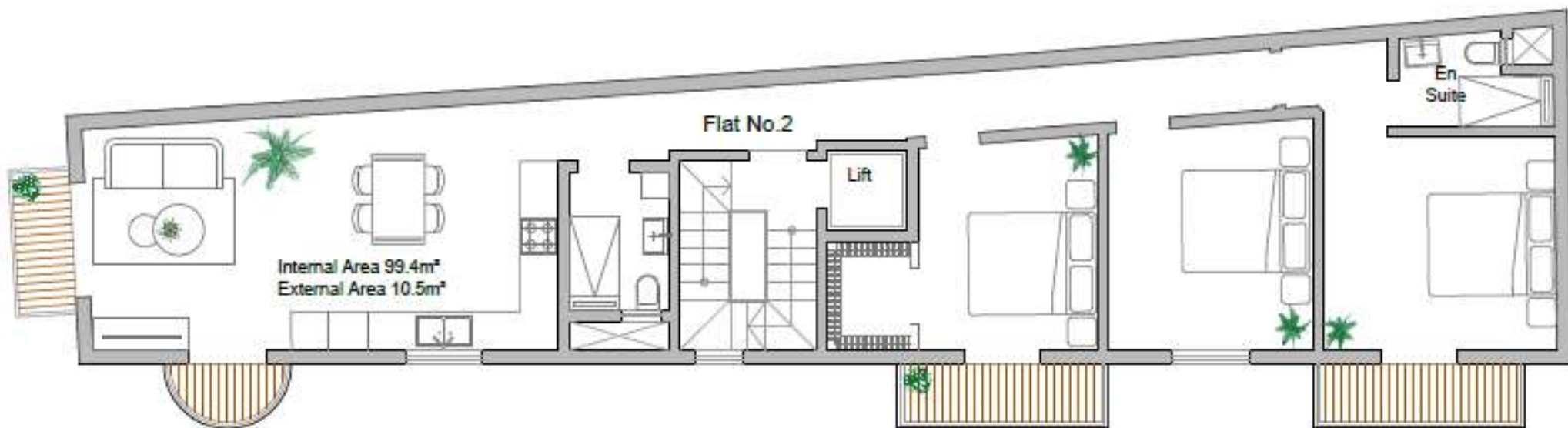
SECOND FLOOR PROPOSED Scale 1:100
