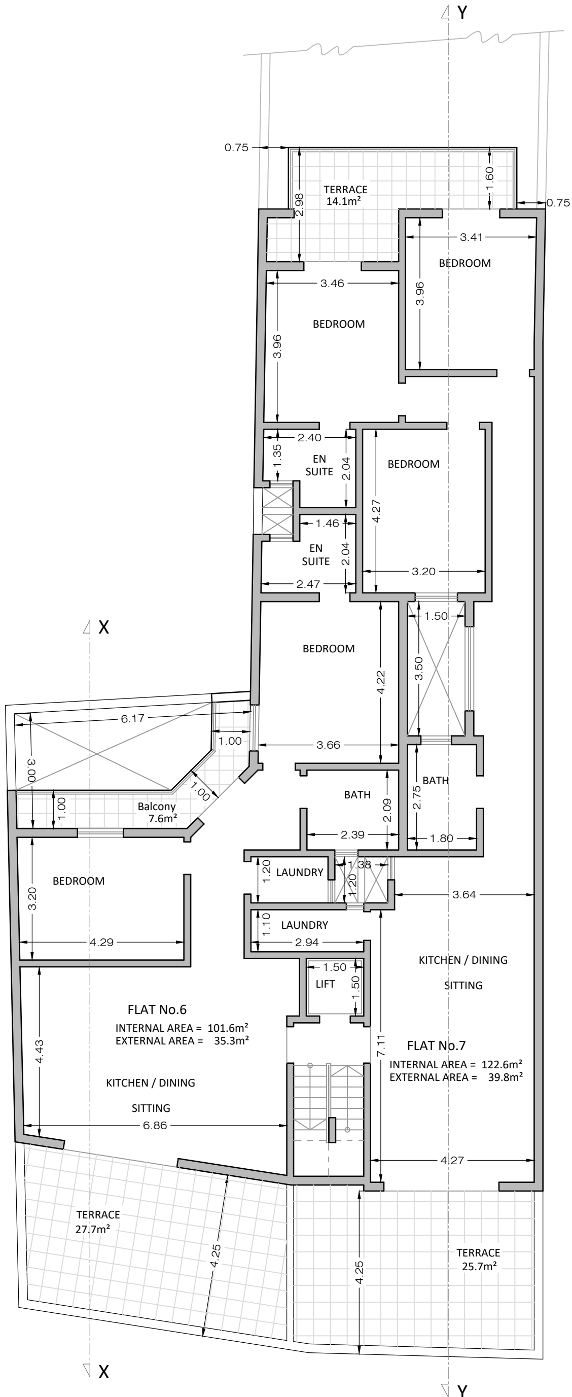
RECEDED FLOOR Scale 1:100
