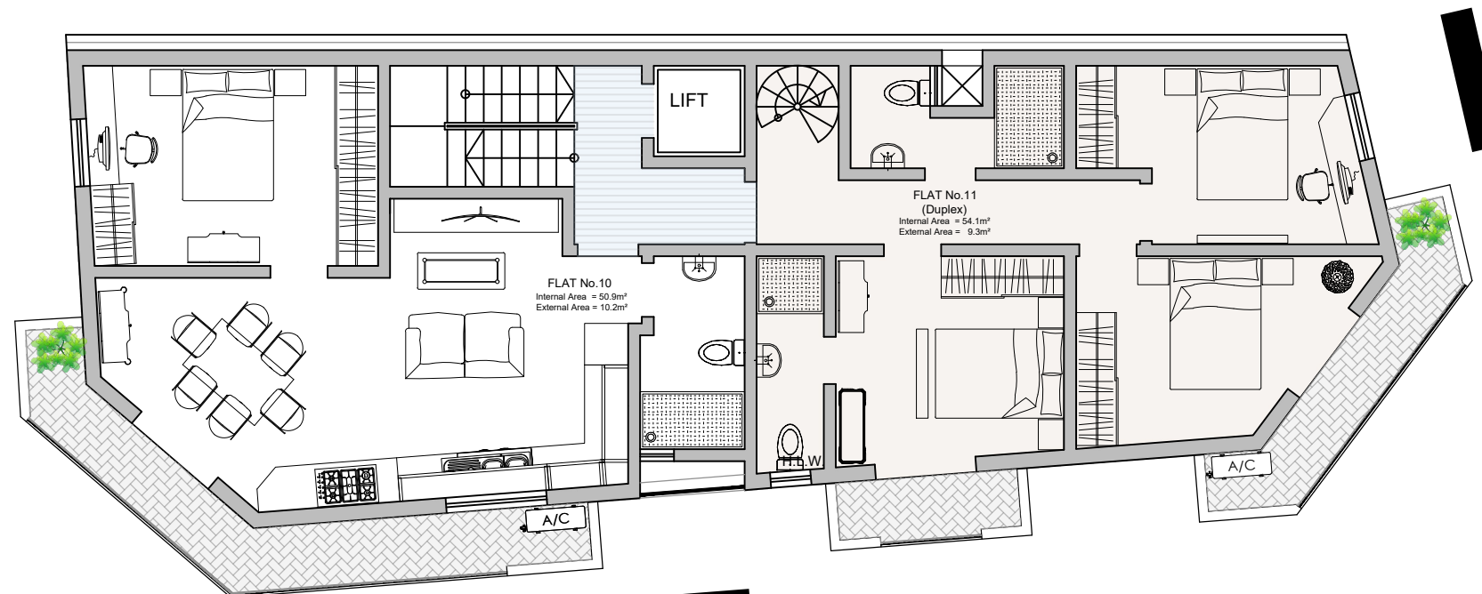
FIFTH FLOOR AS PROPOSED Scale 1:100
