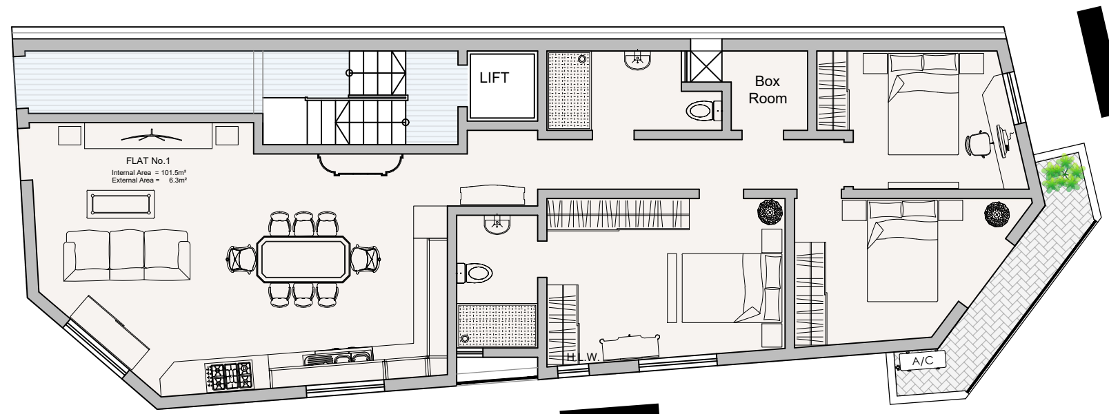
GROUND FLOOR AS PROPOSED Scale 1:100
