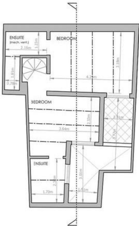
SECOND FLOOR PLAN AS PROPOSED (clean copy) Gross Floor Area 44.8m 2 SCALE 1:100
