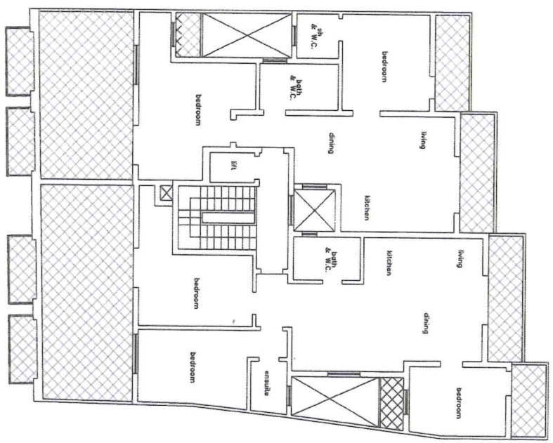
Approved Penthouse level in PA3432/08 Scale 1:100
