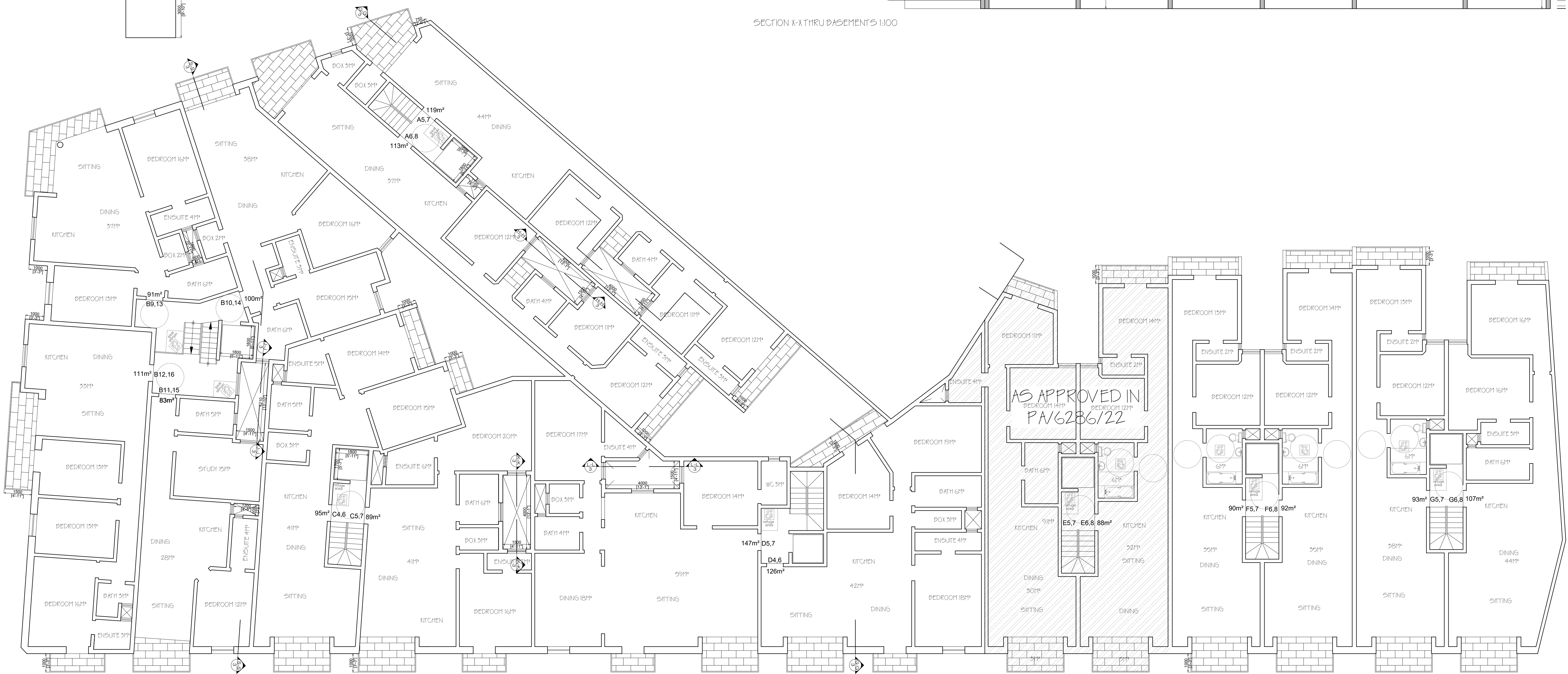
TYPICAL SECOND AND THIRD FLOOR PLAN 1:100
