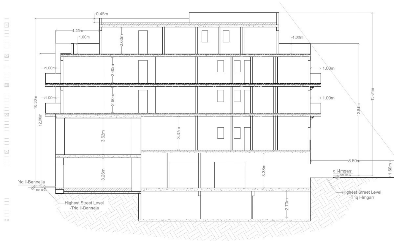
01 Proposed Section C MA30 Clean Copy Scale 1:100 on A1
