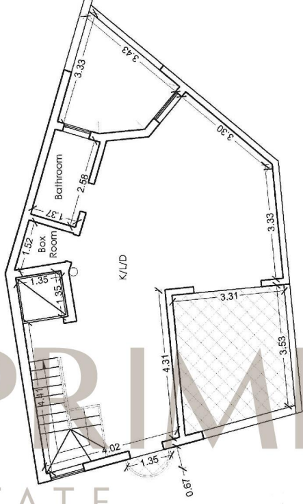
As Proposed Second Floor
