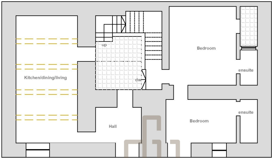
EXISTING ground floor level scale 1:100
