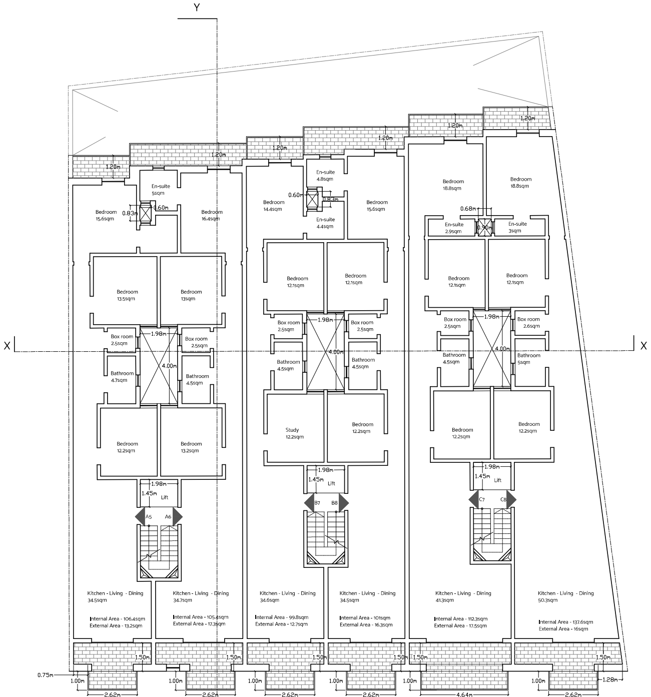
Proposed third floor level plan scale 1:100 dean copy
