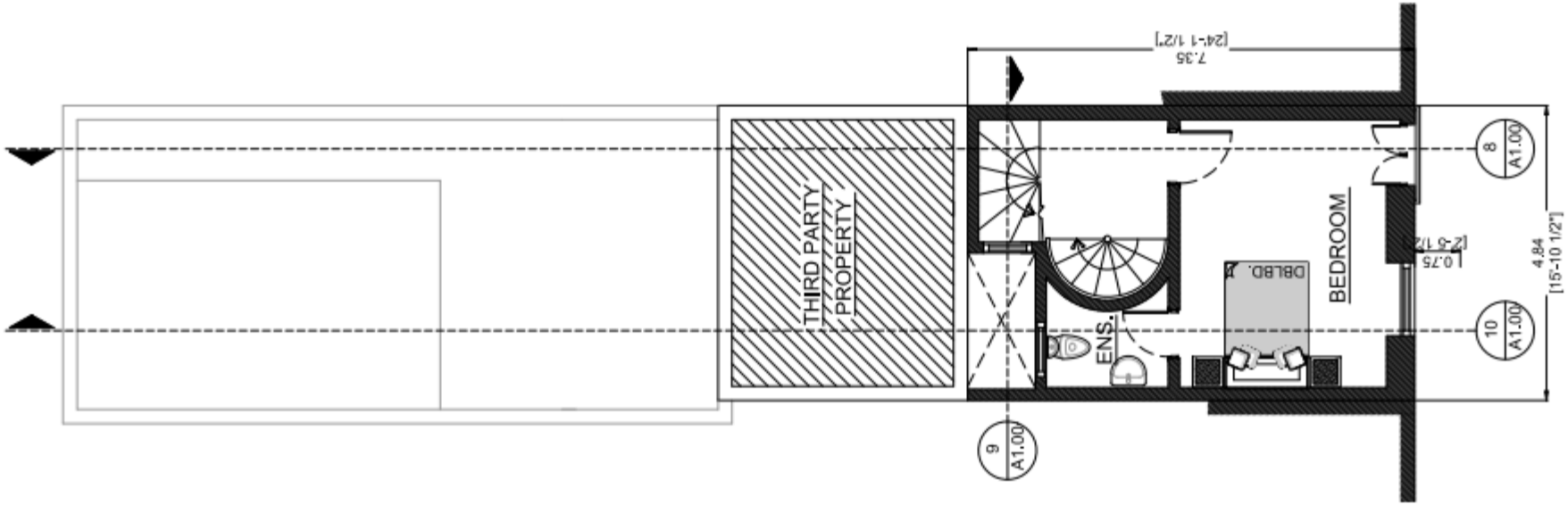
2 PROPOSED FIRST FLOOR SCALE 1:100
