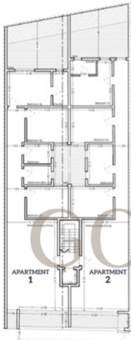
First Floor
