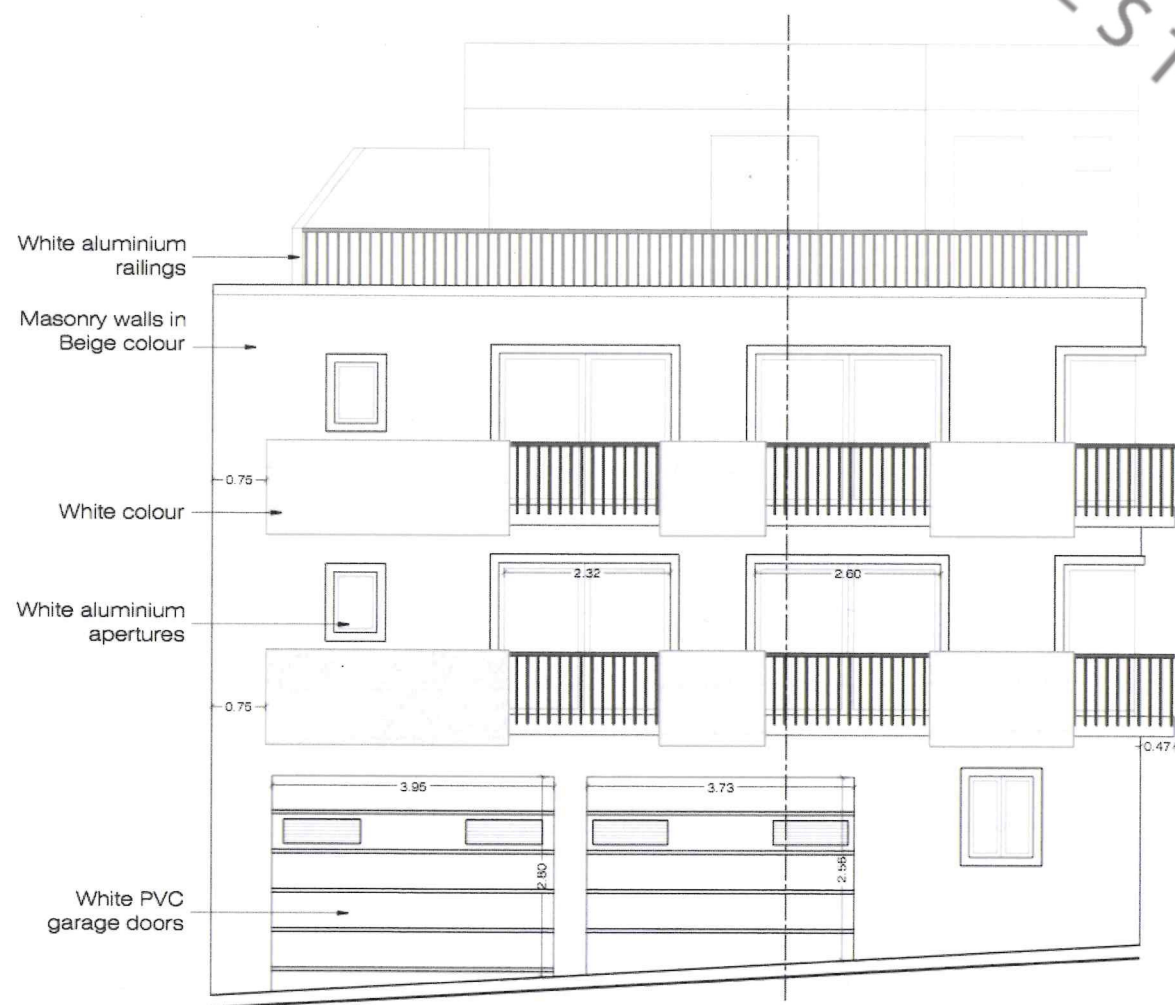
Proposed elevation A Scale 1:50
