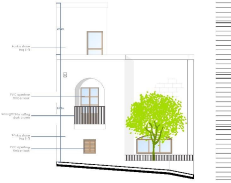
Proposed Front Elevation
